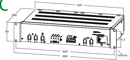
PC1000/2000 Rackmounted 19" 2U. Brackets L89-3 (std)
